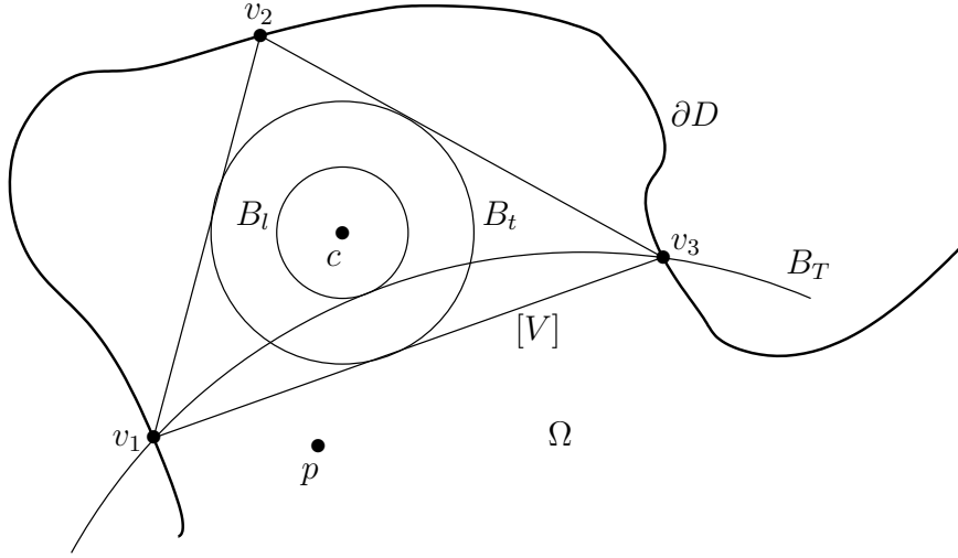
FIGURE 1. The largest ball B_T tangent to B_l and contained in \Omega = \mathbb{R}^n \setminus V , where V = \{v_1, v_2, v_3\} .
