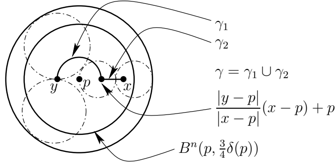
FIGURE 3. A short path \gamma = \gamma_1 \cup \gamma_2 connecting x and y in B^n(p, \frac{3}{4}\delta(p)) .
