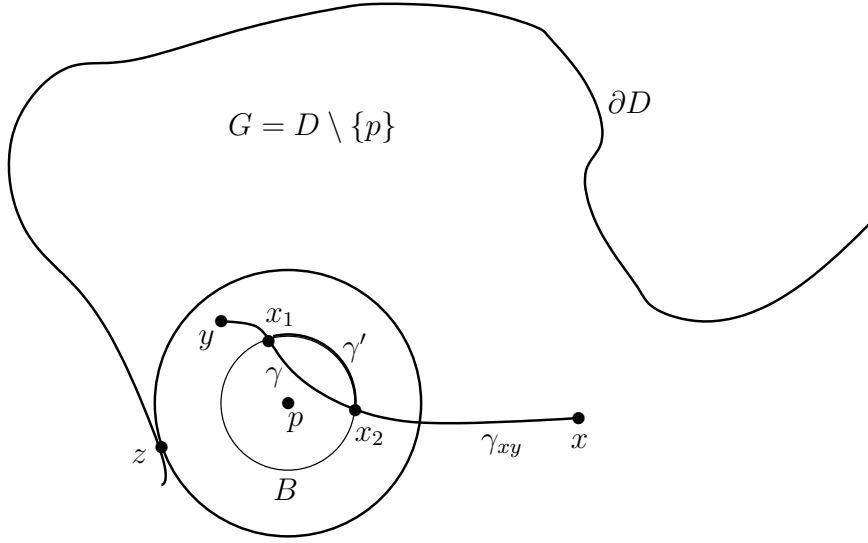
FIGURE 2. The geodesic path \gamma_{xy} (w.r.t. the Apollonian inner metric \tilde{\alpha}_D ) connecting x and y intersects B , and its modification \gamma' from x_1 to x_2 along the circular part.
