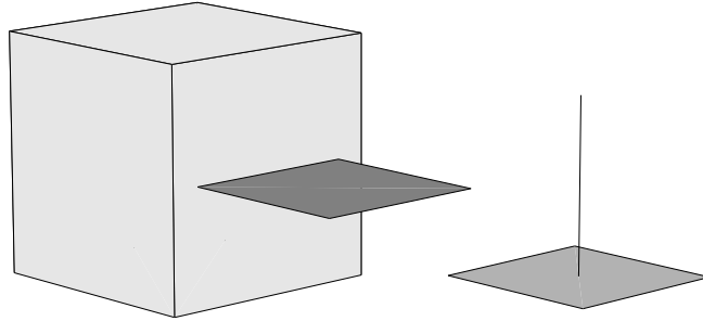
Figure 1. Some metric spaces
