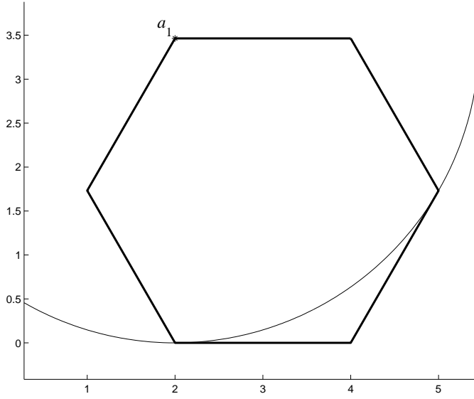
FIGURE 3. The minimum is not attained at the vertices.
