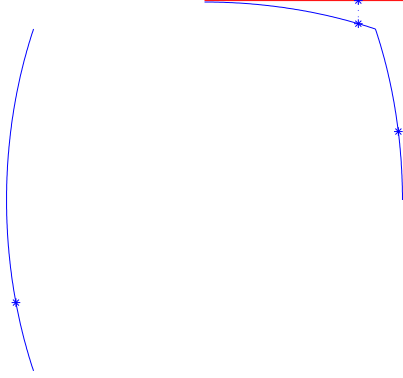
FIGURE 6. A set of constant 3-diameter.
