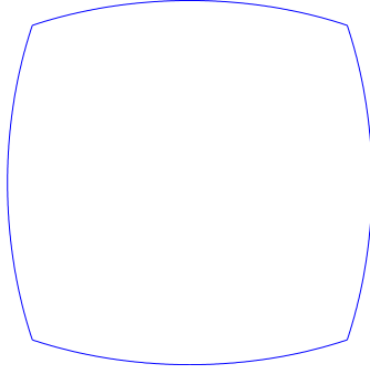
FIGURE 5. A set of constant 3-diameter.
