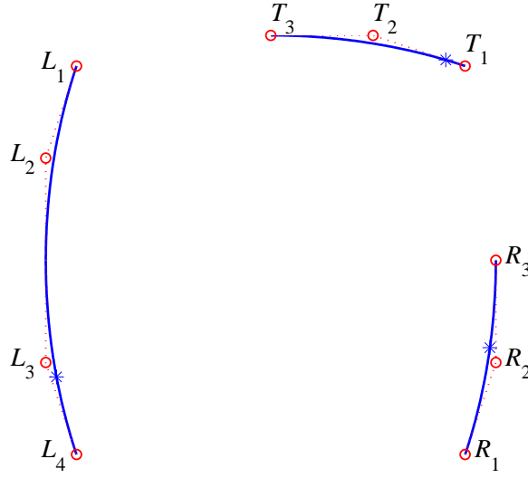
FIGURE 7. A set of constant 3-diameter.
