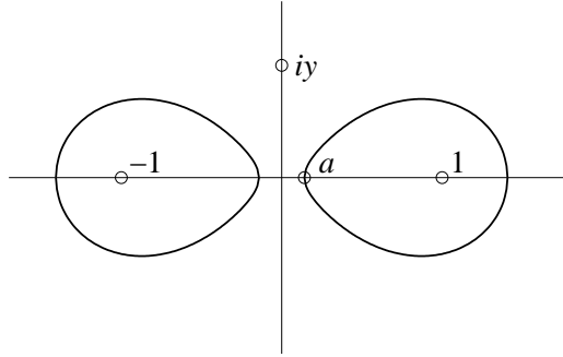
FIGURE 4. The set E from Proposition 4.5
